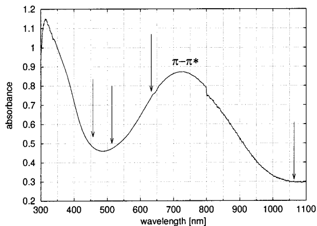
Figure 8. UV-vis spectrum of pDdT3, neutral form. Arrows indicate the excitation wavelengths for Raman measurements.
