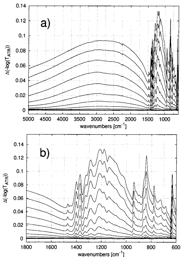
Figure 5. IR difference spectra of pDdT3 during oxidation. Sequence: bottom to top. (a) extended range; (b) IRAV range.
