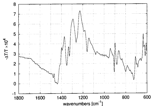
Figure 7. PIA-FTIR spectrum of pDdT3, neutral form. Excitation at 488 nm, 30 mW/cm 2 .
