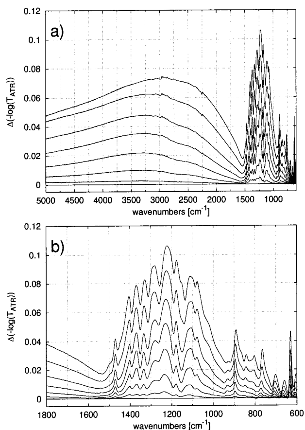
Figure 6. IR difference spectra of pDdT3 during reduction. Sequence: bottom to top. (a): extended range; (b): IRAV range.
