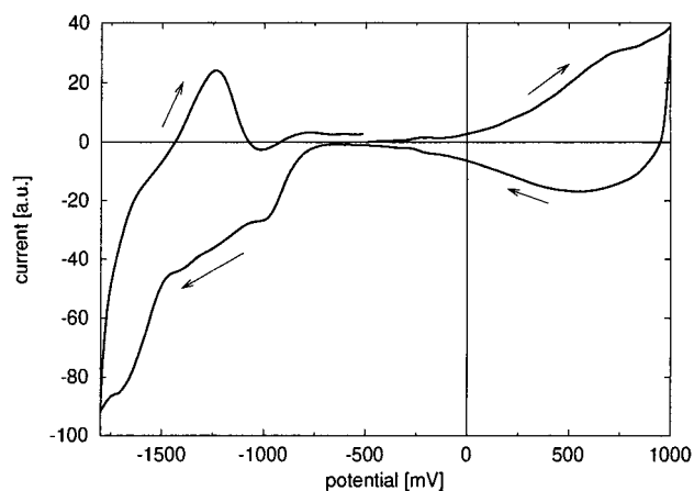
Figure 4. Cyclic voltammogram during the in situ spectroelectrochemical experiment. Electrolyte 0.1 M Bu 4 NPF 6 in CH 3 CN, sweep rate 5 mV/s.
