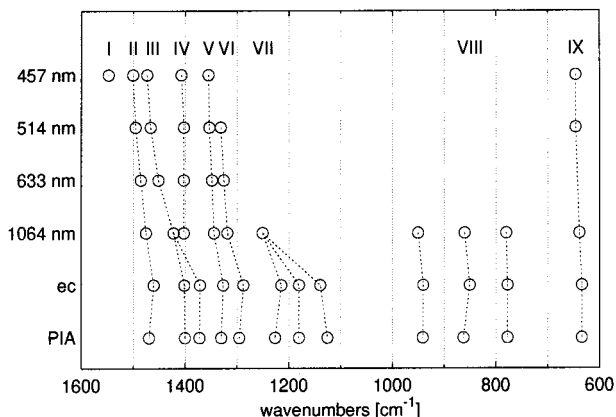
Figure 10. Outline of the Raman bands and correlation to IR/V bands of pDdT3. Roman numbers are band numbers, wavelength for Raman excitation, ec electrochemical oxidation, PIA photoinduced IR absorption.
