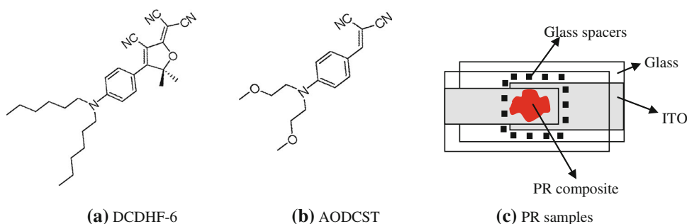
Fig. 1 Molecular structure of DCDHF-6 (a) and AODCST (b). c Scheme of the photorefractive polymer composite beam combiner
