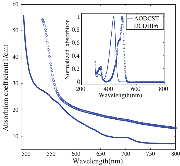
Fig. 2 Absorption coefficient of the polymer composites DCDHF-6:PVK:BBP:PCBM (circles) and AODCST:PVK:BBP:PCBM (line) between 500- and 800-nm wavelength. Inset normalized absorption of the composites in solution
