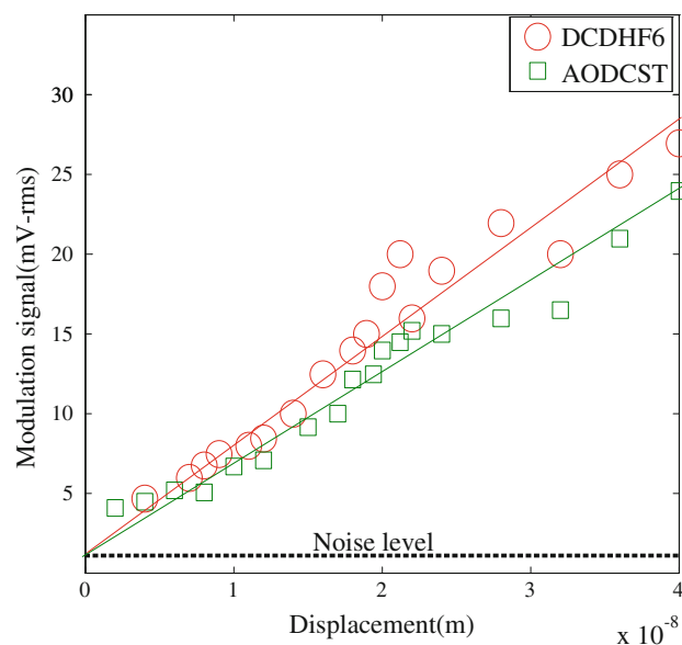
Fig. 5 Amplitude of the modulated signals received by PR detectors based on DCDHF-6 and AODCST as a function of the applied ultrasonic amplitude at 100 Hz
