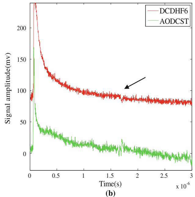
Fig. 7 Measured longitudinal echoes detected in transmission geometry on (a) an aluminum sheet with 3 mm thickness (b) on a 9-mm-thick steel sample using DCDHF-6:PVK:BBP:PCBM (red lines) and AODCST:PVK:BBP:PCBM (green lines) photorefractive polymer interferometers at 50 V/ \mu\text{m}
