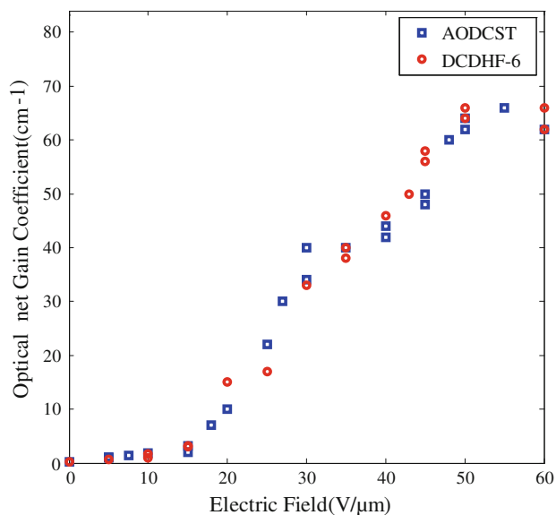
Fig. 4 Optical net gain coefficient versus applied electric field for AODCST/PVK/C60/BBP (squares) and DCDHF-6/PVK/C60/BBP (circles)
