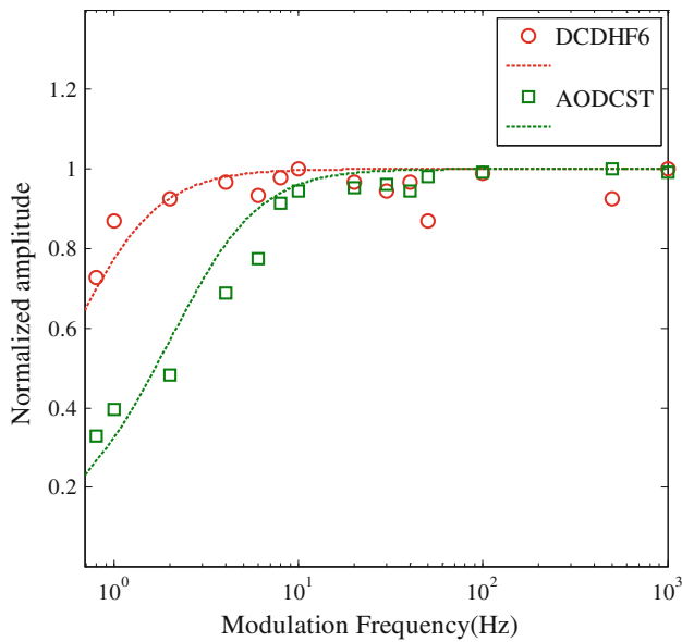
Fig. 6 Modulated amplitudes as a function of frequency for LUS detector based on DCDHF-6 (circles) and AODCST (squares) PR polymer composites. The dashed lines display fits to the experimental data
