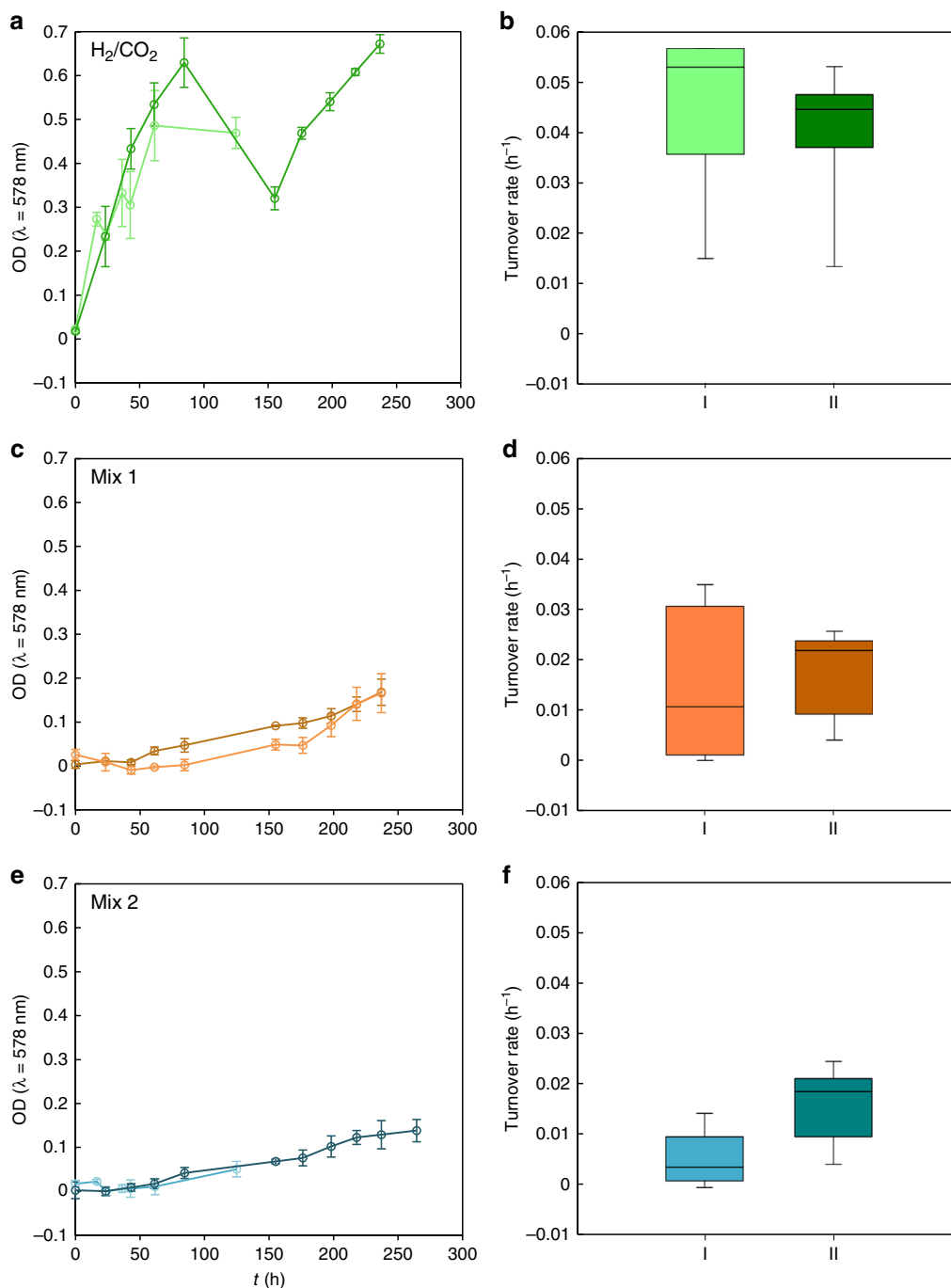
Fig. 3 Growth and turnover rate of M. okinawensis under Enceladus-like conditions at 2 bar. a, c, e Growth curves ( OD_{578 \text{ nm}} ) and b, d, f turnover rates ( h^{-1} ) as a measure of CH_4 production of M. okinawensis on a, b H_2/CO_2 (4:1), c, d Mix 1 and e, f Mix 2. For detailed composition of gases and media see Table 2 and Supplementary Table 3. I and II (light and dark colours, respectively) denote two independent experiments (each performed in triplicates, error bars = standard deviation). Enceladus-like concentrations were used for NH_4Cl and CH_3OH and mean liquid inhibitor concentrations determined in the DoE were used for CH_2O . The dip in a was caused by substrate limitation due to depletion of serum bottle headspace of H_2/CO_2 at high-optical cell densities
